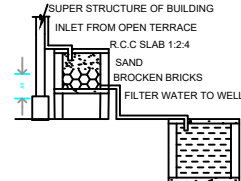
RAINWATER HARVESTING
