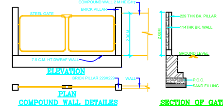
COMPOUND WALL DETAILS
