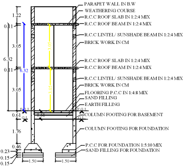
SECTION ON-AA
