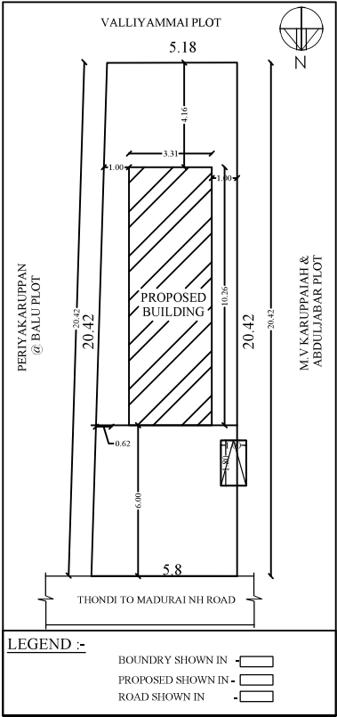
SITE PLAN
