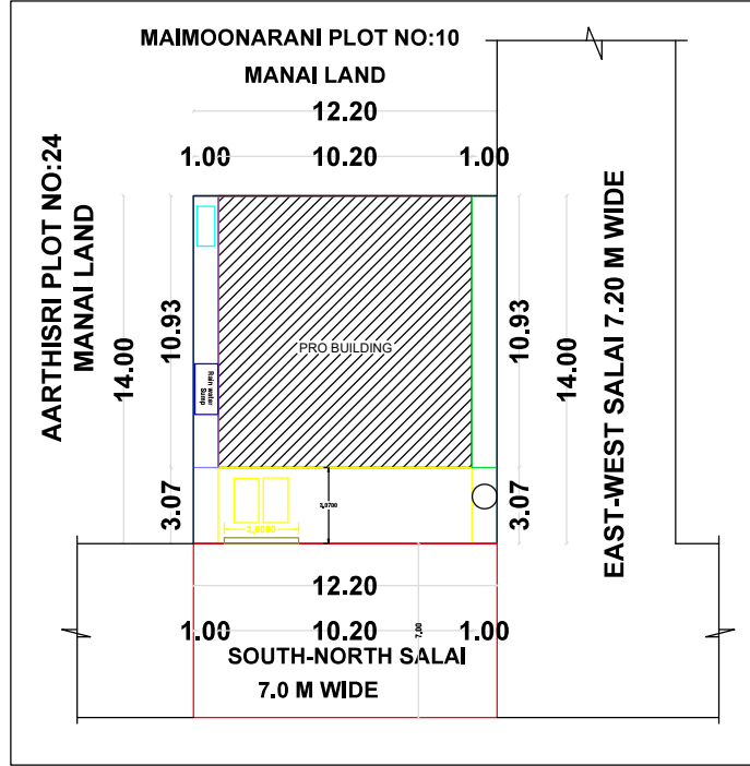
SITE PLAN & KEY PLAN
