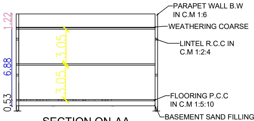
SECTION ON-AA
