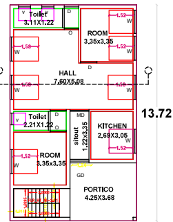
GROUND FLOOR PL
