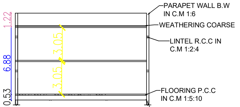
SECTION ON-AA
