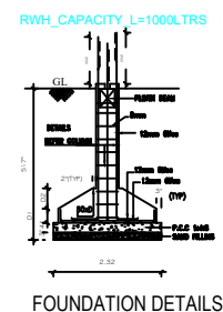
FOUNDATION DETAILS
