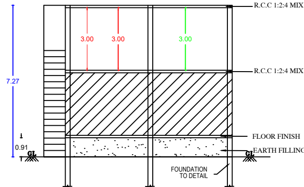
SECTION AB
