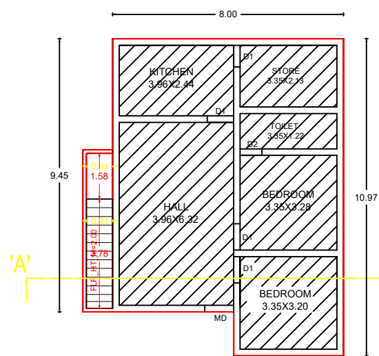
EXI GROUND FLOOR PLAN
