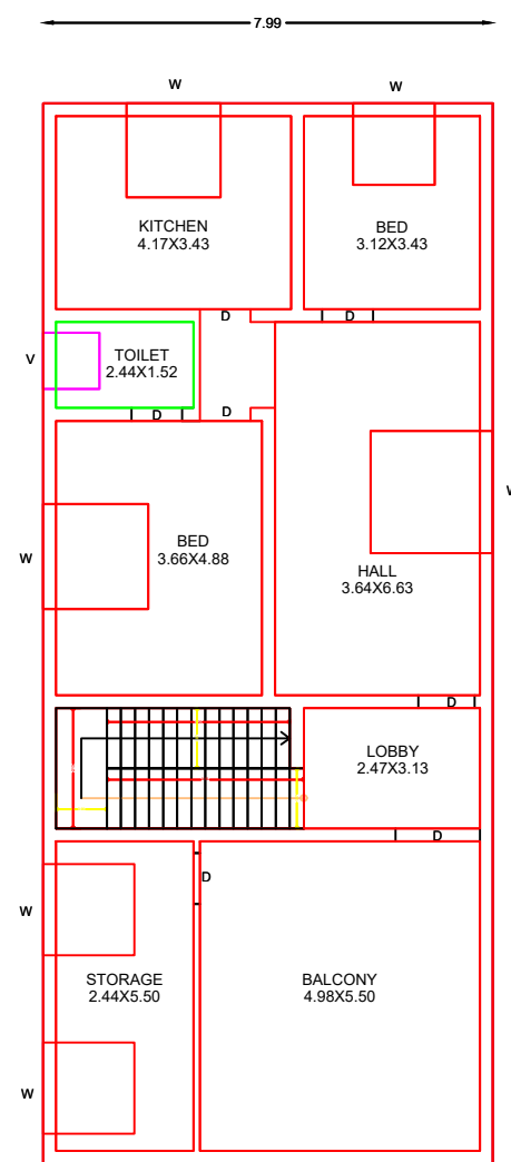
PROPOSED RESIDENTIAL FIRST FLOOR PLAN
