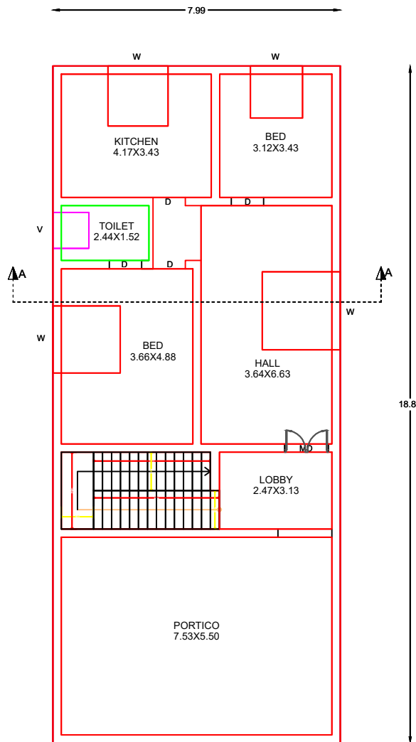
PROPOSED RESIDENTIAL GROUND FLOOR PLAN
