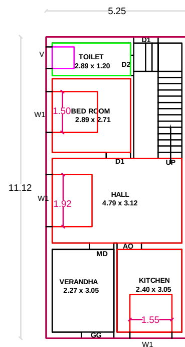
GROUND FLOOR PLAN PROPOSED
