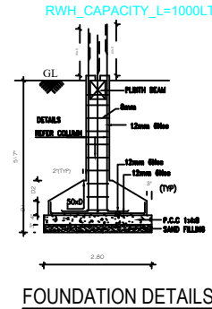
FOUNDATION DETAILS
