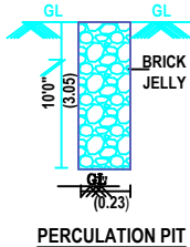
PERCOLATION PIT
