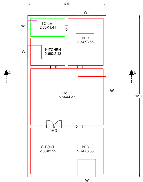
PROPOSED RESIDENTIAL GROUND FLOOR PLAN
