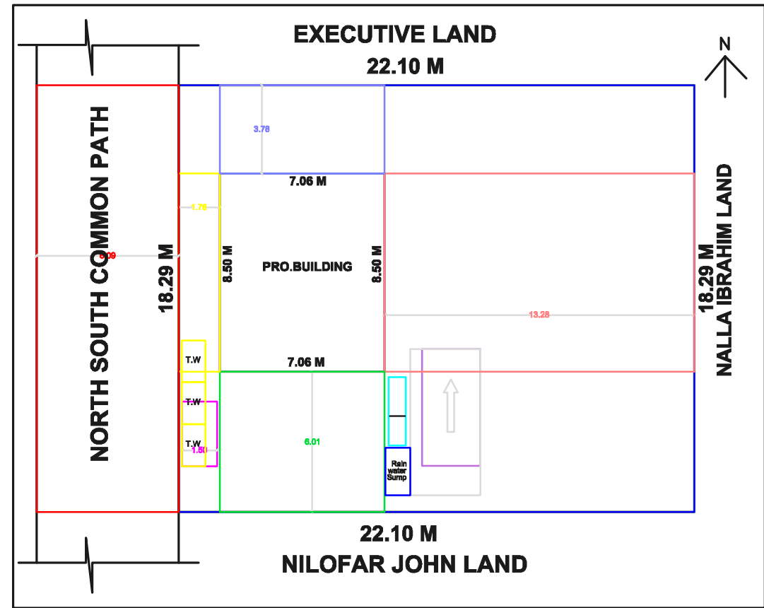
SITE PLAN
