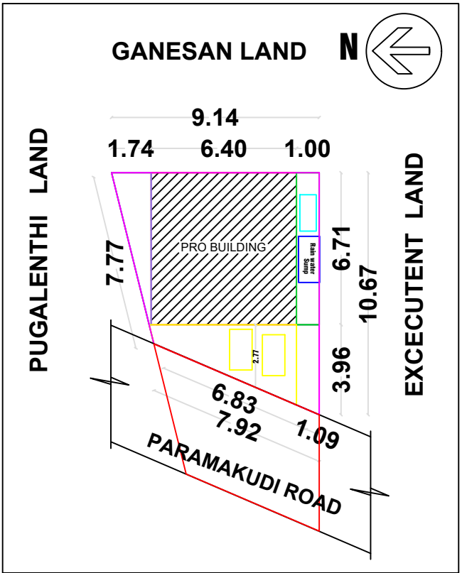
SITE PLAN & KEY PLAN
