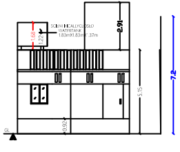
FRONT ELEVATION
