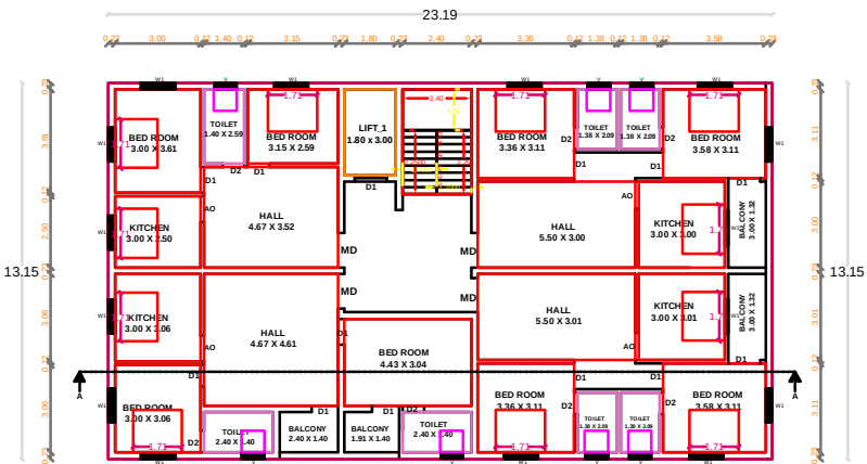
SECOND FLOOR PLAN PROPOSED
