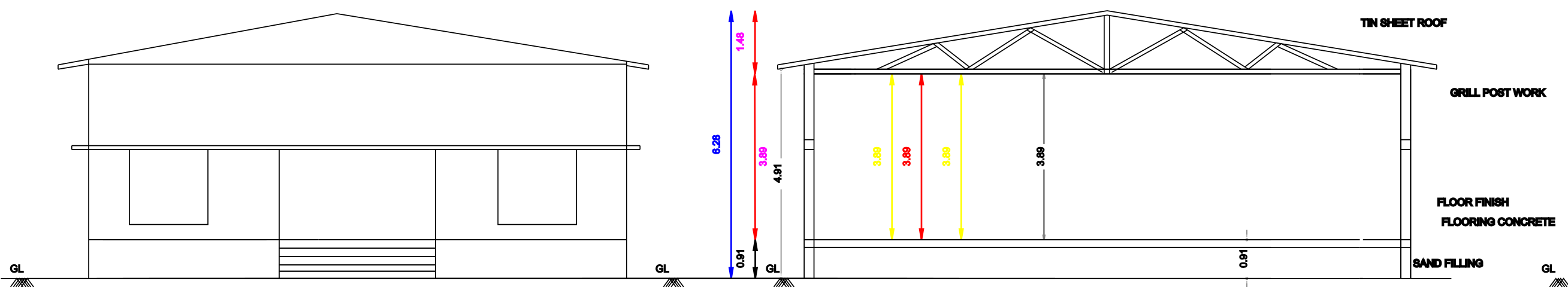
SECTION ON AB
