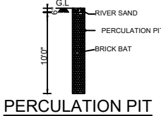
PERCOLATION PIT
