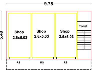
PRO. GROUND FLOOR PLAN
