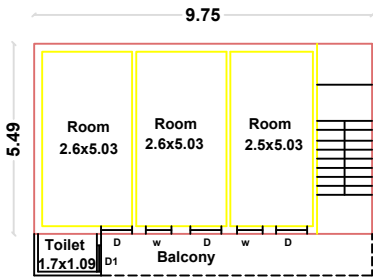
PRO. FIRST FLOOR PLAN
