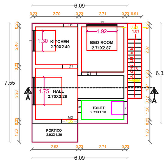
GROUND FLOOR PLAN PROPOSED
