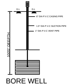
BORE WELL
