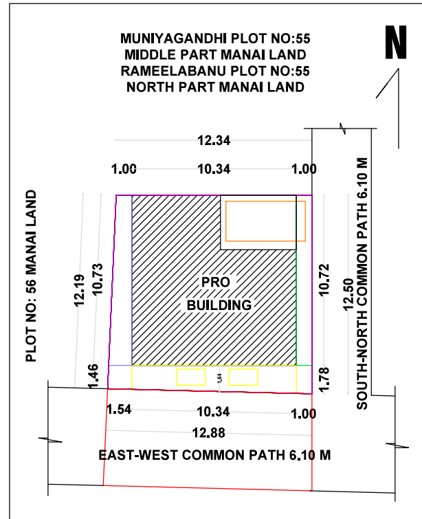
SITE PLAN & KEY PLAN
