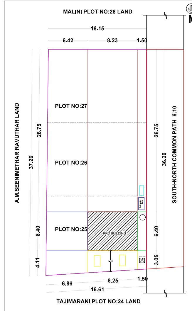
SITE PLAN & KEY PLAN
