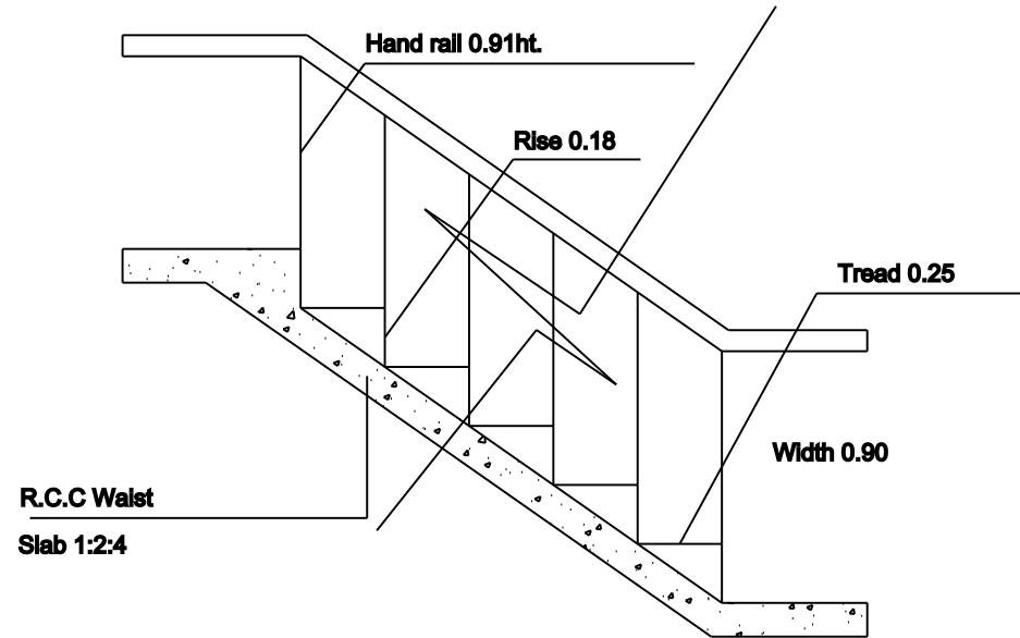
STAIRCASE DETAIL
