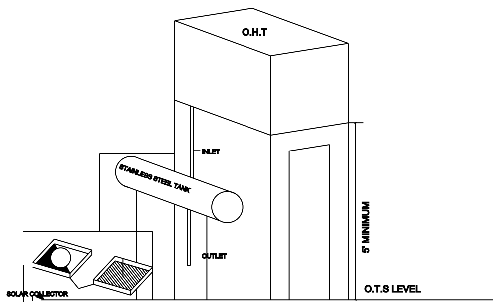
SOLAR WATER HEATER
