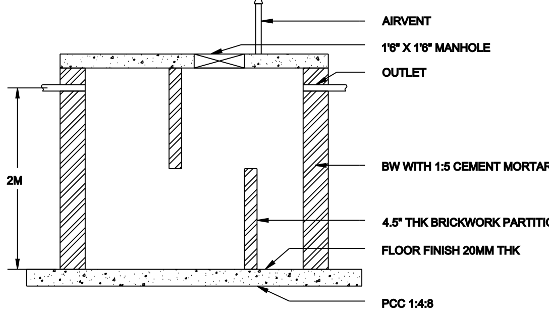
CROSS SECTION OF SEPTIC TANK
