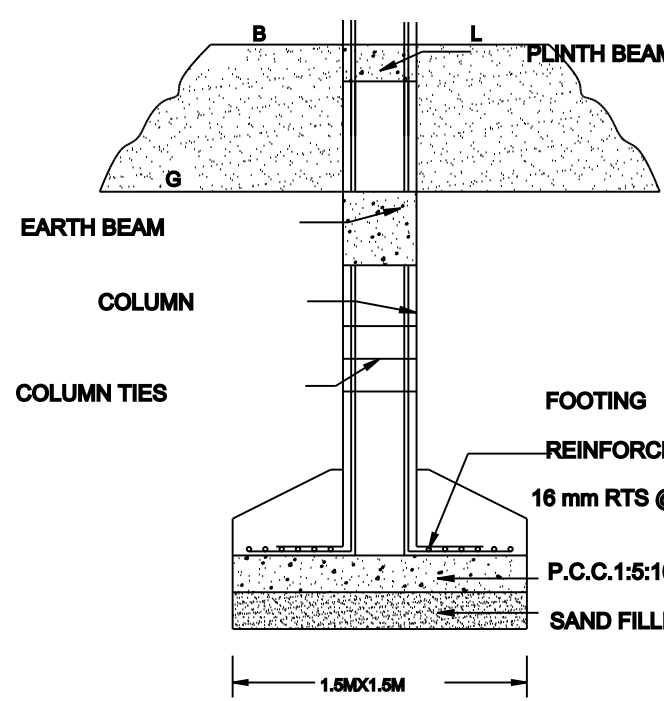
FOUNDATION DETAIL
