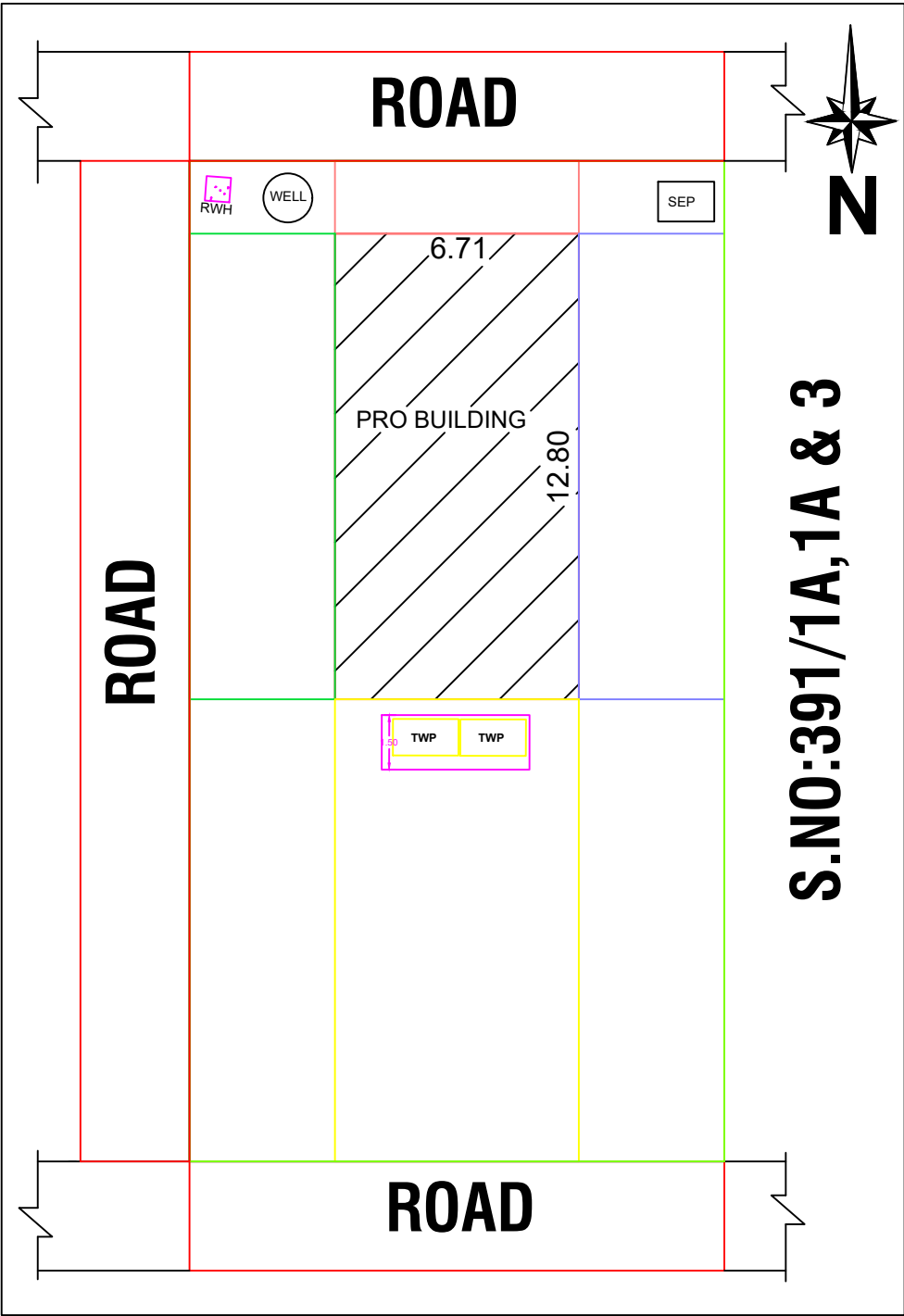
SITE PLAN
