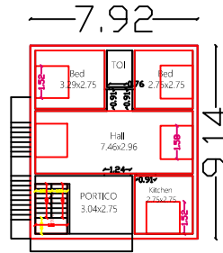
SITE PLAN AND GROUND FLOOR PLAN
