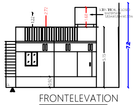
FRONT ELEVATION
