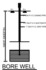
BORE WELL
