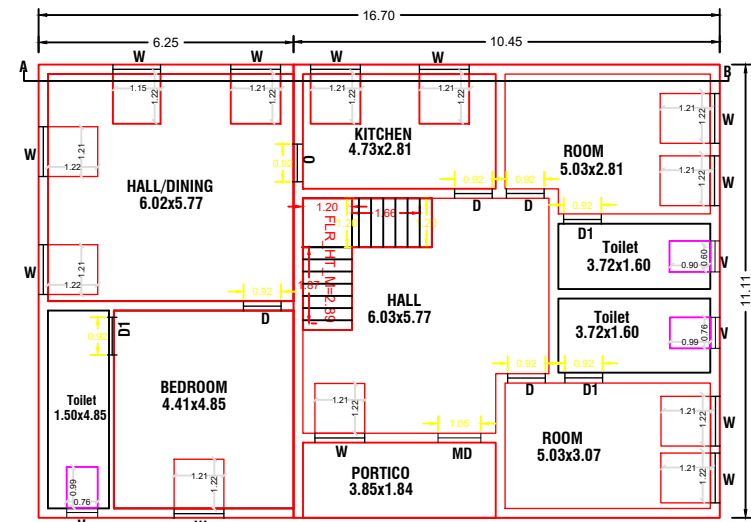
ADDITIONAL GROUND FLOOR PLAN EXISTING., GROUND FLOOR PLAN
