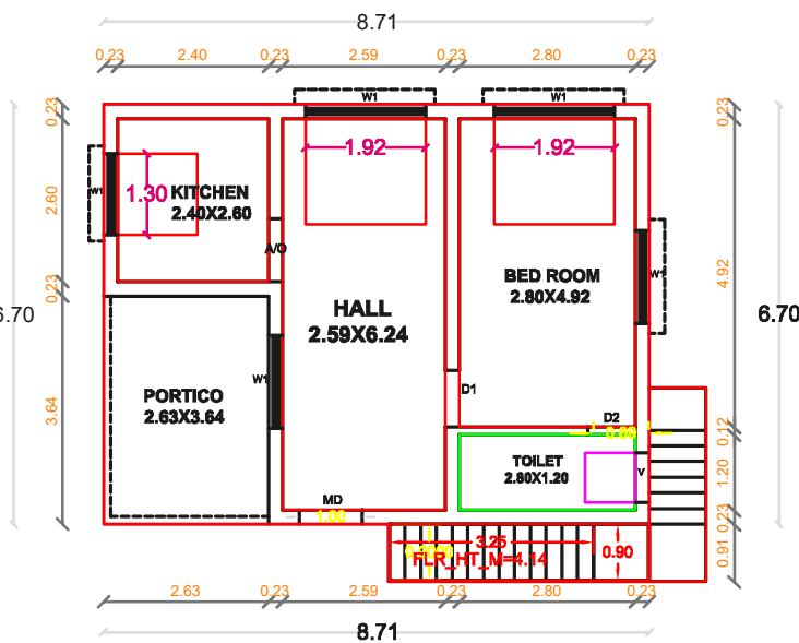
GROUND FLOOR PLAN PROPOSED
