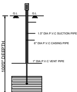
BORE WELL
