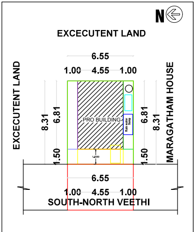
SITE PLAN & KEY PLAN
