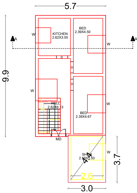
EXISTING RESIDENTIAL GROUND FLOOR BUILDING & PROPOSED COMMERCIAL GROUND FLOOR PLAN
