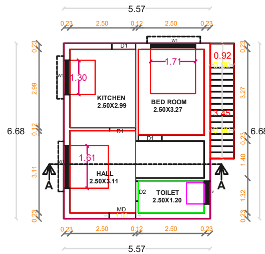
GROUND FLOOR PLAN PROPOSED
