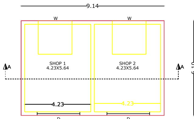
PROPOSED COMMERCIAL GROUND FLOOR PLAN
