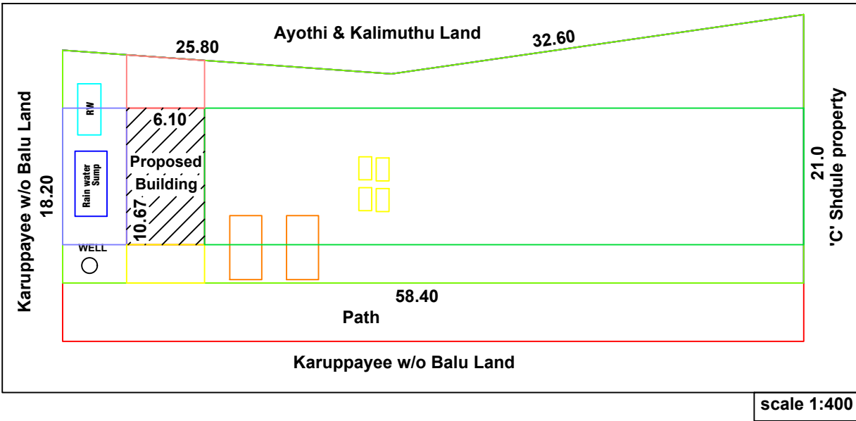
SITE PLAN CUM KEYPLAN
