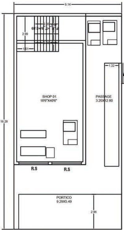
ADD., GROUND FLOOR PLAN
