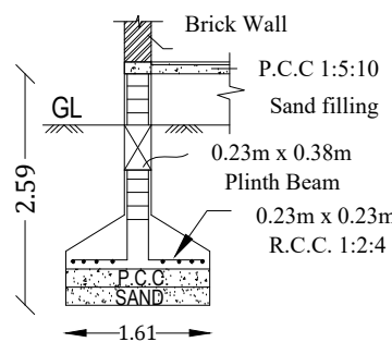
FOUNDATION DETAILS
