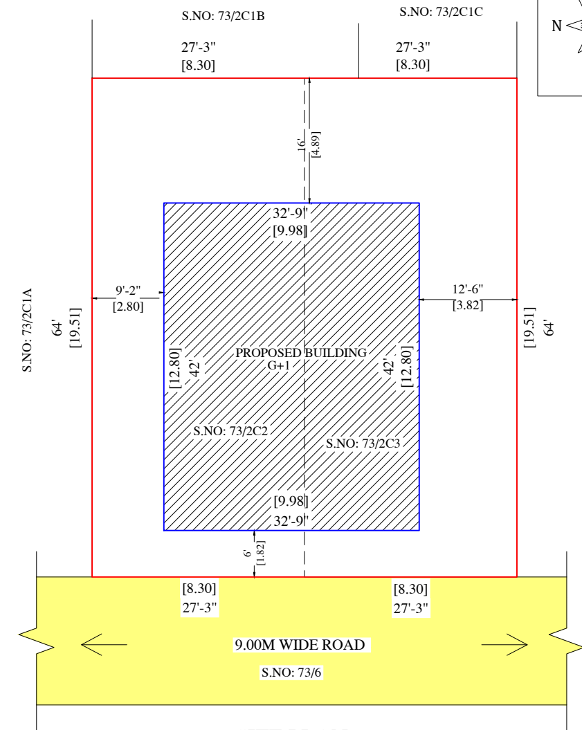
SITE PLAN
