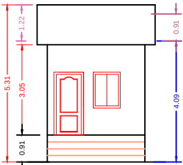
FRONT ELEVATION
