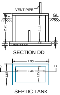
SEPTIC TANK
