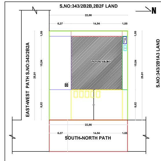
SITE PLAN CUM KEYPLAN
