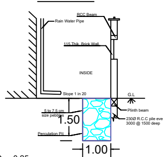
Percolation Pit
