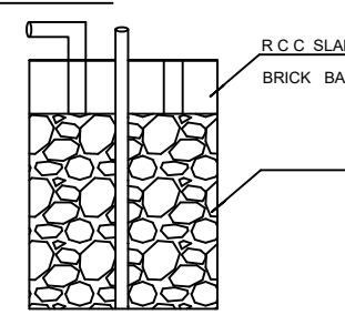
RAIN WATER STORAGE
