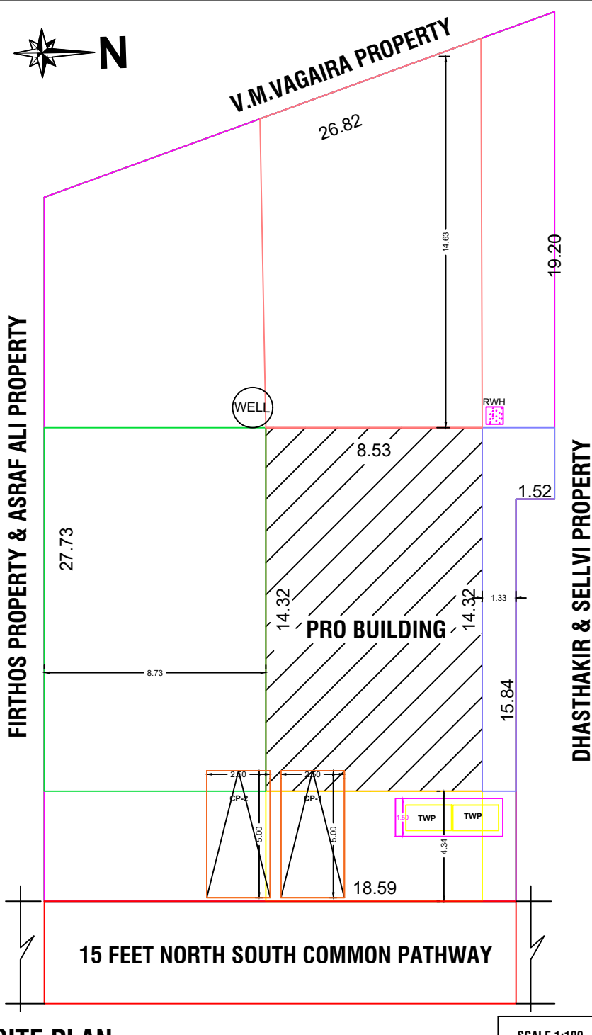
SITE PLAN
