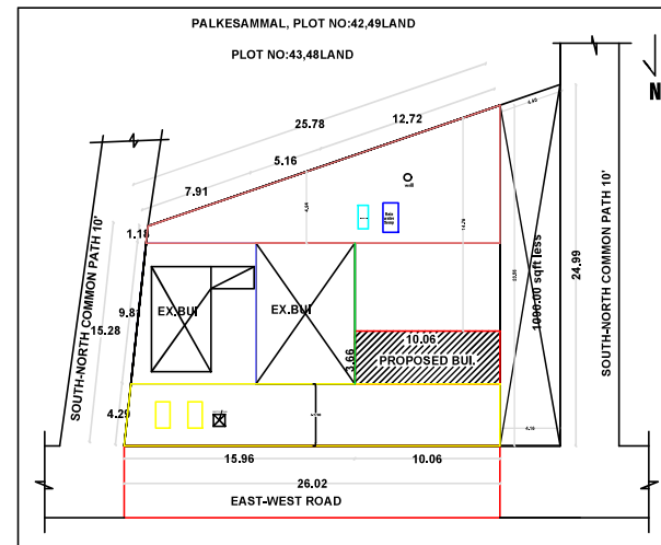
SITE PLAN & KEY PLAN
