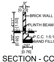
SECTION - CC
