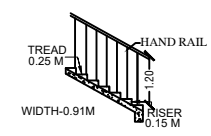
STAIRCASE DETAILS
