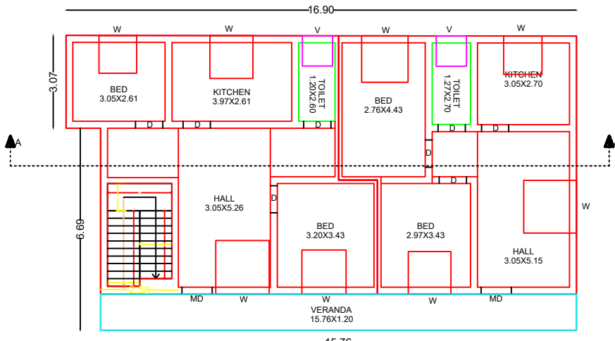
PROPOSED RESIDENTIAL FIRST FLOOR PLAN
