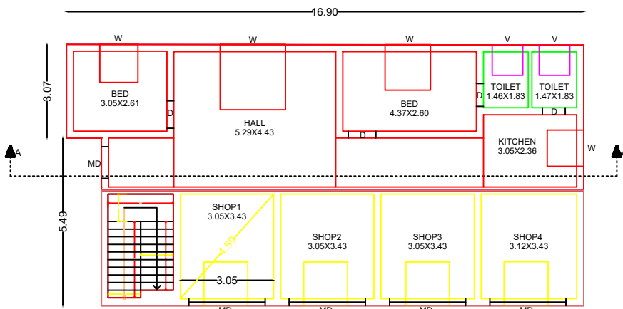
PROPOSED COMMERCIAL & RESIDENTIAL GROUND FLOOR PLAN
