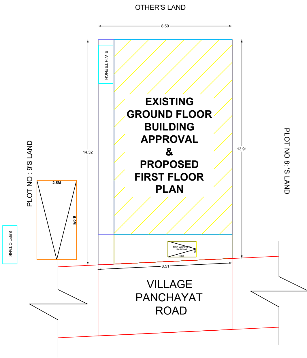
SITE PLAN
