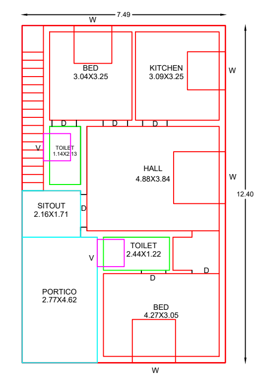
EXISTING GROUND FLOOR BUILDING
