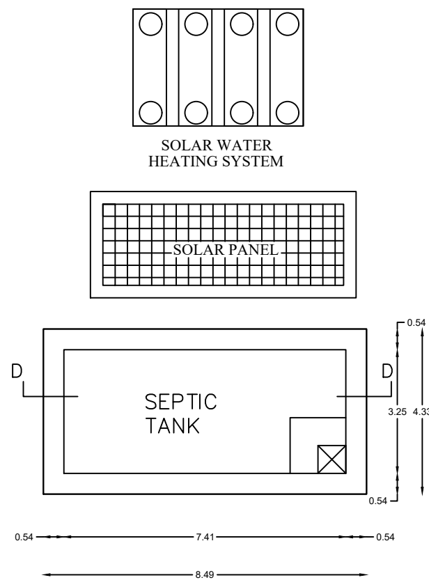
PLAN OF SEPTIC TANK SCALE 1"=2'0"
