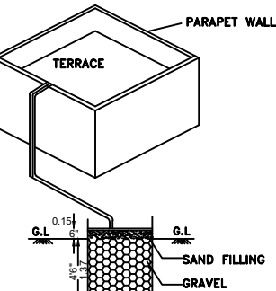
COLLECTION OF SUMP RAINWATER HARVESTING FROM TERRACE
