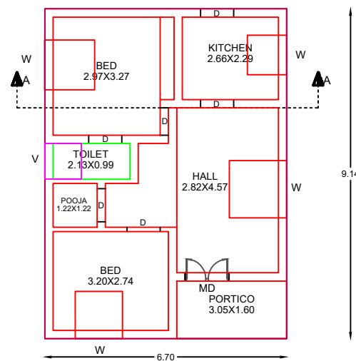
PROPOSED RESIDENTIAL GROUND FLOOR PLAN
