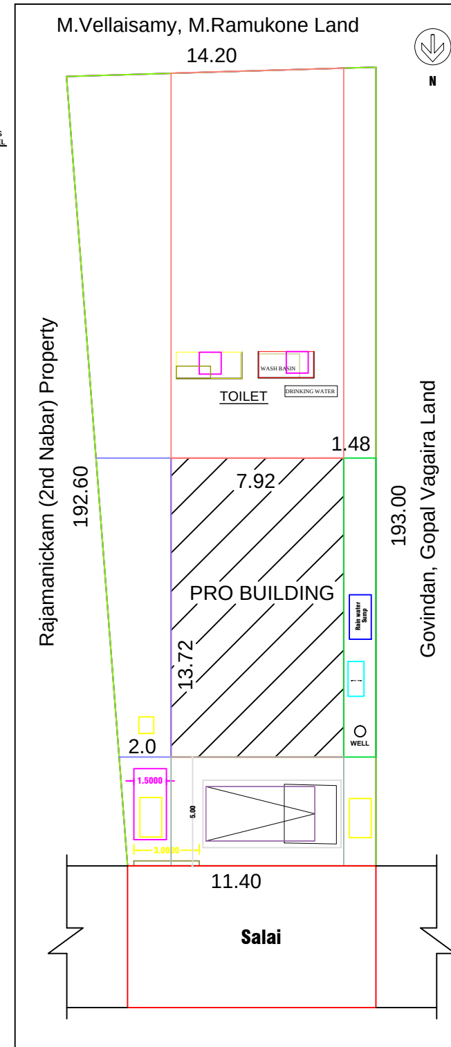
SITE PLAN & KEY PLAN
