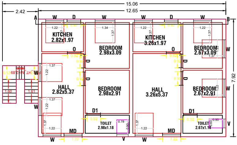
PRO., GROUND FLOOR PLAN
