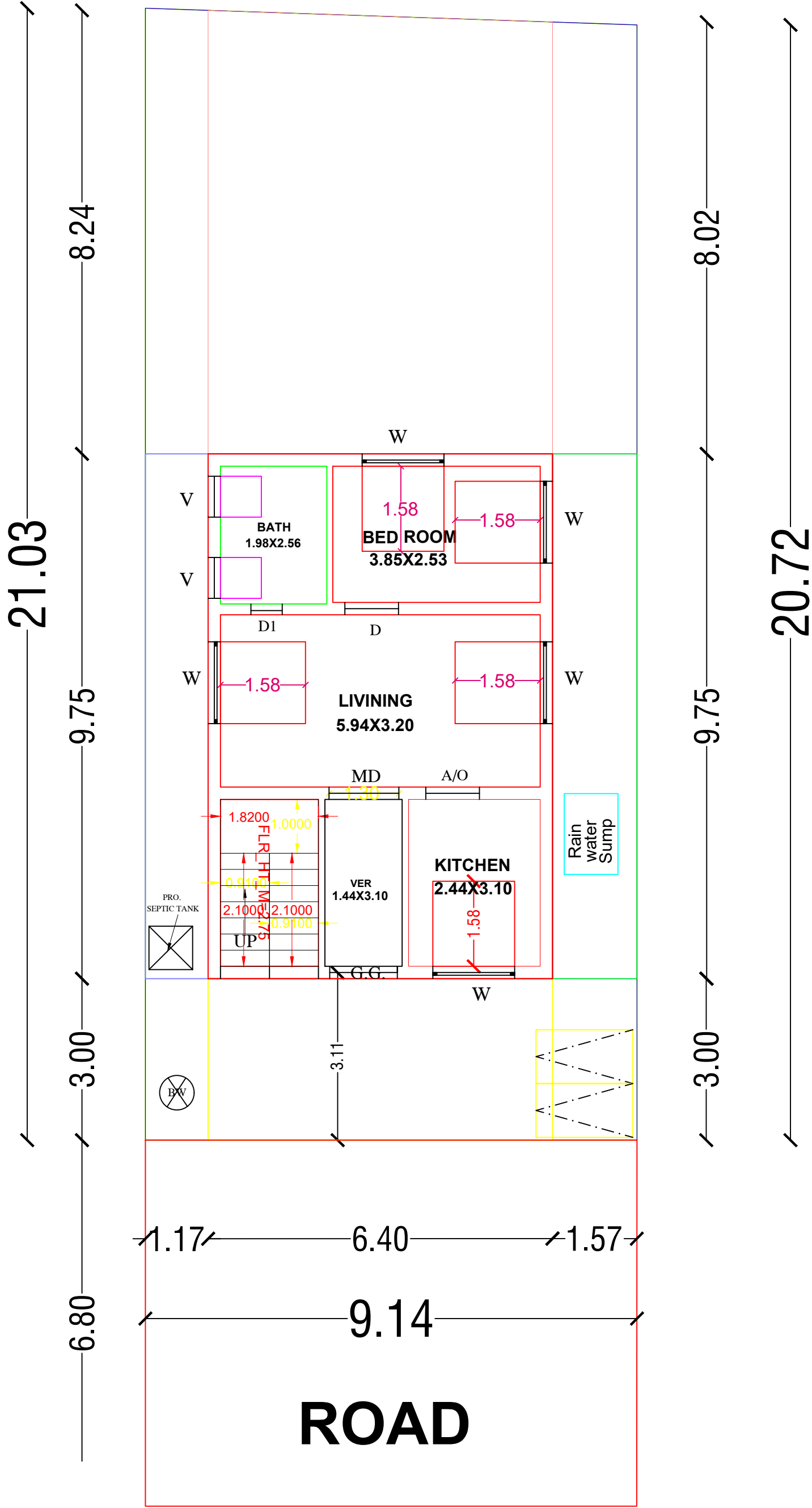
PLAN CUM GROUND FLOOR PLAN
