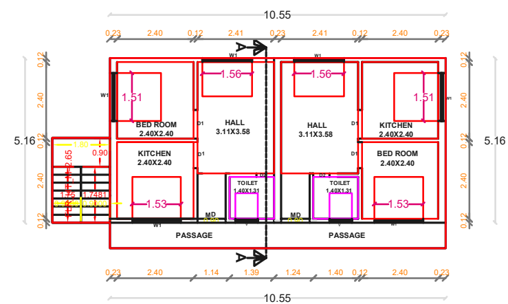
FIRST FLOOR PLAN (PROPOSED)
