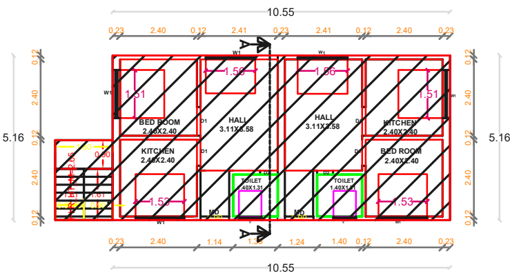
GROUND FLOOR PLAN (EXISTING)
