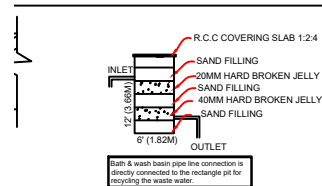
RAIN WATER HARVESTING SYSTEM
