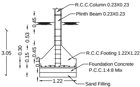
DETAILS OF COLUMN FOOTING (SCALE 1:50)
