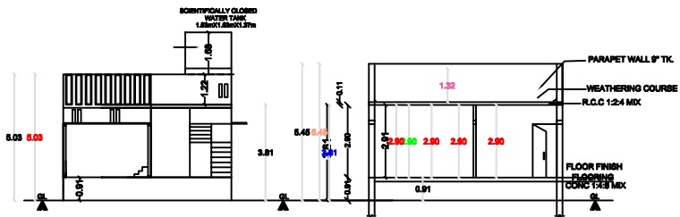
FRONT ELEVATION
